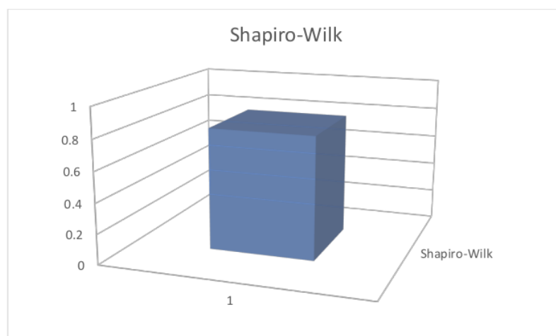
Figura 12. Shapiro Wilk
